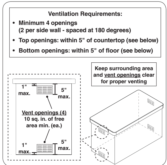
Fig. 11-1 Ventilation detail
