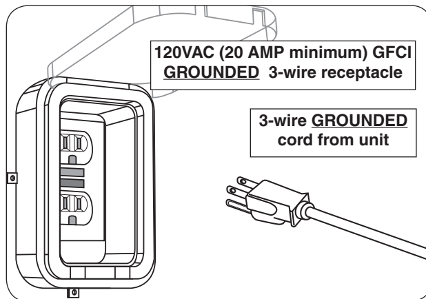
Fig. 17-2 Connect power cord
