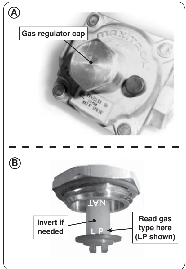
Fig. 23-1 Convert regulator
