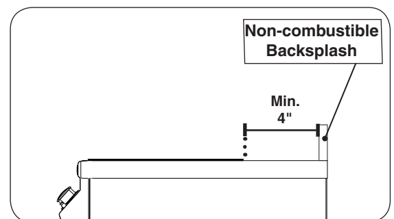
Fig. 9-5 Backsplash clearance
