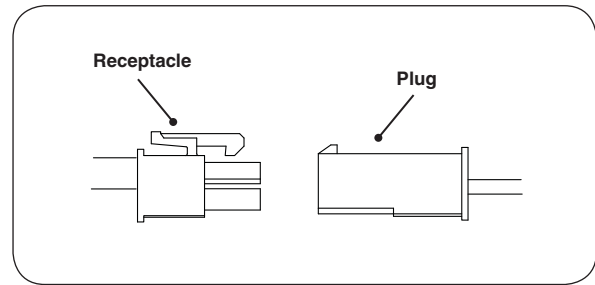
Fig. 16-1 Connection detail
