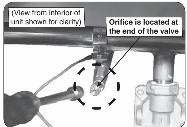
Fig. 24-3 Orifice location
