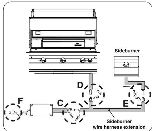
Fig. 16-3 Connect sideburner to grill setup
