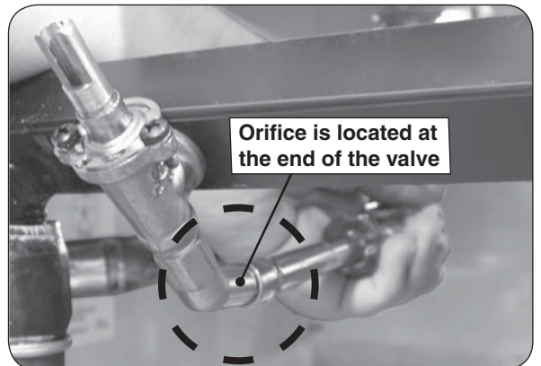
Fig. 26-3 Single sideburner orifice location
