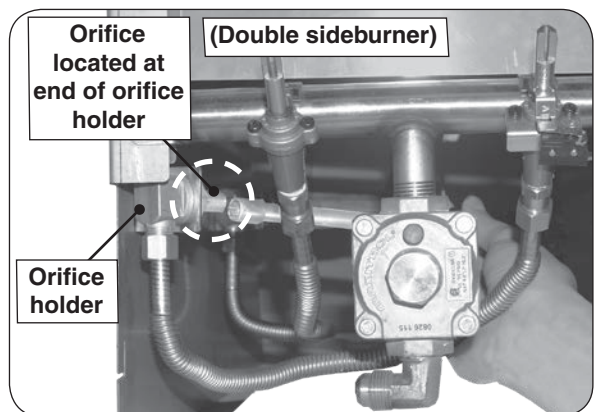
Fig. 26-4 Double sideburner orifice locations
