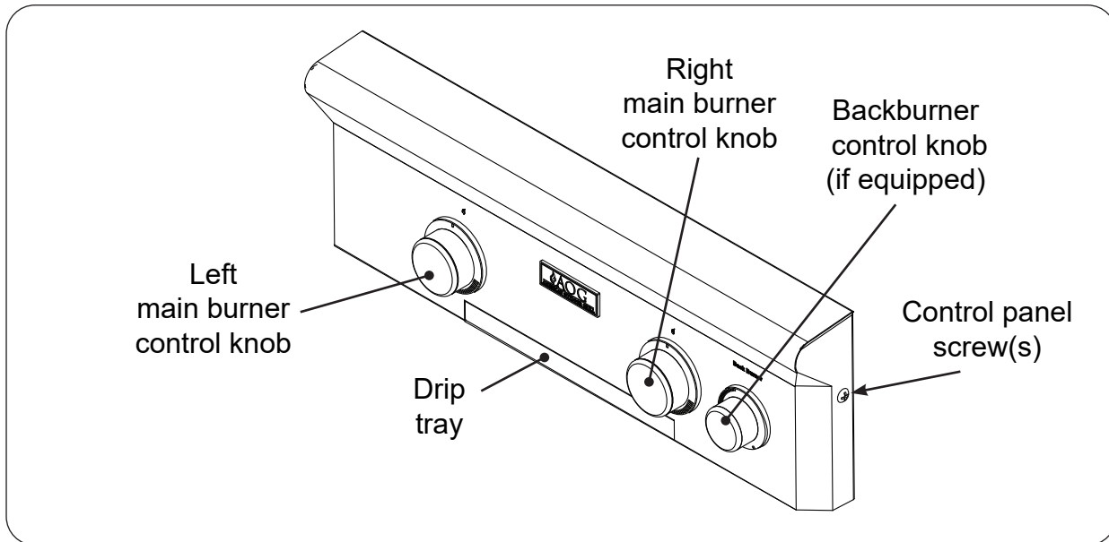
Fig. 29-1 24" model controls
