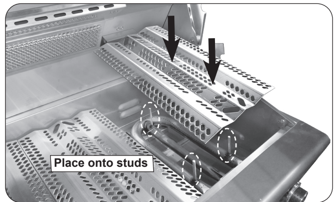
Fig. 27-1 Install vaporizer panels
