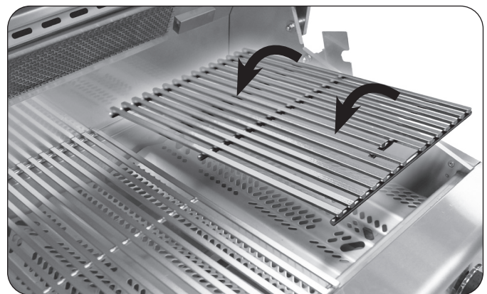
Fig. 27-2 Install cooking grids
