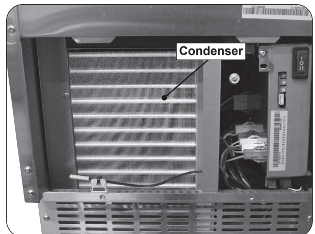
Fig. 13-4 Clean condenser
