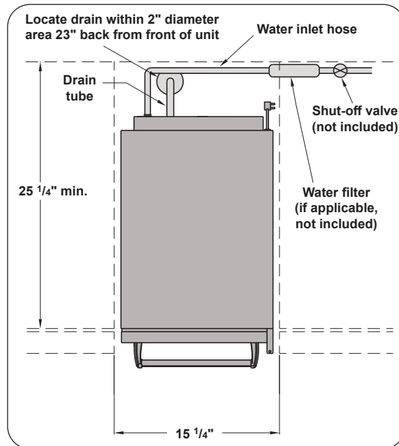
Fig. 9-1 Top view
