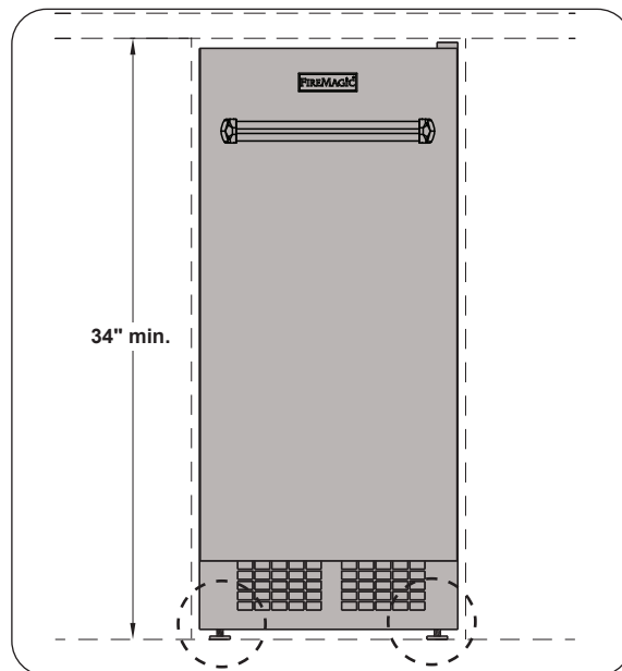
Fig. 9-2 Front view
